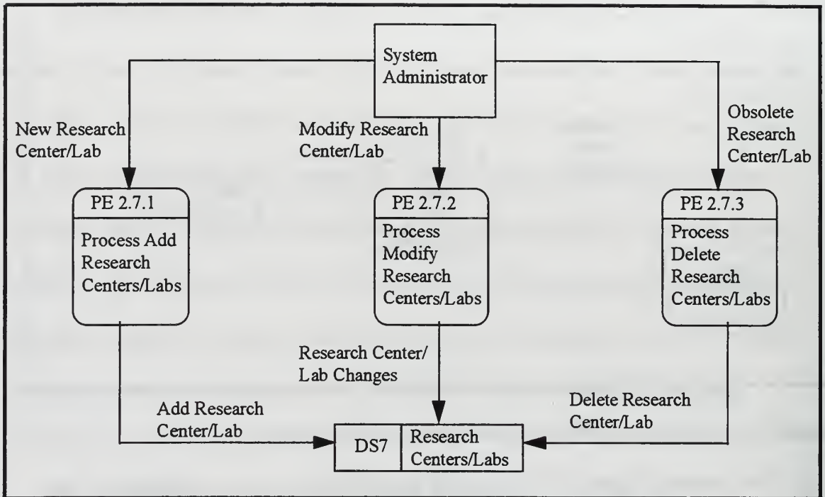
Figure 14. Primitive Level DFD For Maintaining Research Centers/Labs
